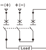
DC 750V (3P)
