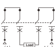
DC 1000V (4P)
