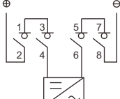
4 Pole in series
