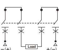
DC 1500V (4P)
